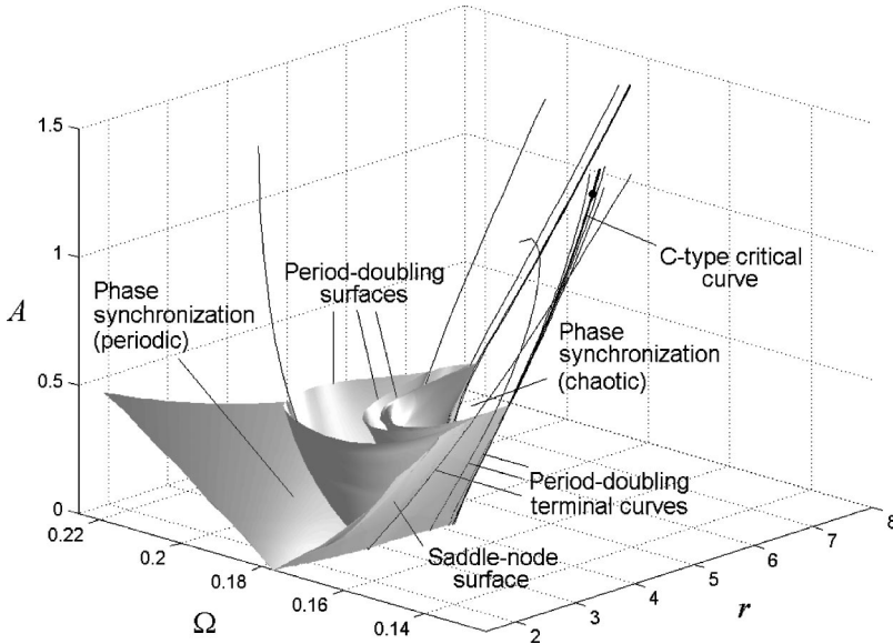
FIG. 1. Three-dimensional view of the parameter space (\Omega, r, A) for the periodically driven Rössler oscillator. The inscriptions explain the nature of the regimes and bifurcations. For clarity of the diagram the bifurcational surfaces are drawn only partially. A point on the critical curve selected for detailed study is marked by a bullet.
