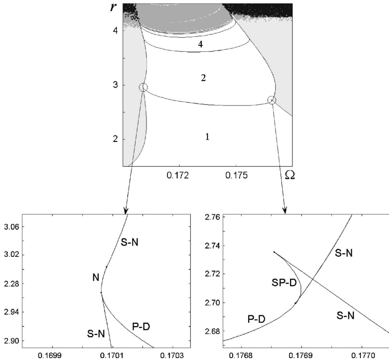
FIG. 2. Bifurcation diagram for the periodically driven Rössler oscillator on the parameter plane (\Omega, r) , at A=0.1 . The white area in the middle is the synchronization zone. Light gray areas correspond to quasiperiodic regimes, dark gray areas at the top to phase synchronization of chaos, and black areas to asynchronous chaotic dynamics. Insets show details of the bifurcational structure near the terminal points of the period-doubling curves marked as P-D . The subcritical period-doubling bifurcation line is designated as SP-D , the bifurcation lines of saddle-node (tangent) bifurcations are designated as S-N , and those of Neimark bifurcations as N .
